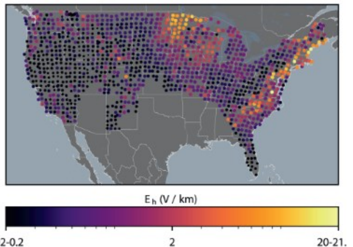
(a) Peak geoelectric amplitudes
