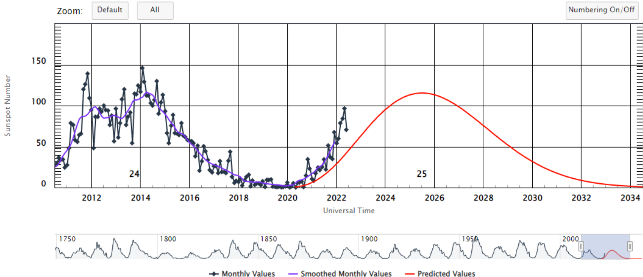
ISES Solar Cycle Sunspot Number Progression
